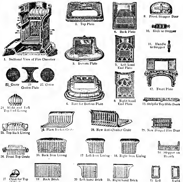
Figs. 3075-3105. NAMES AND NUMBERS OF PARTS OF THE SPEAR CABOOSE STOVE.
